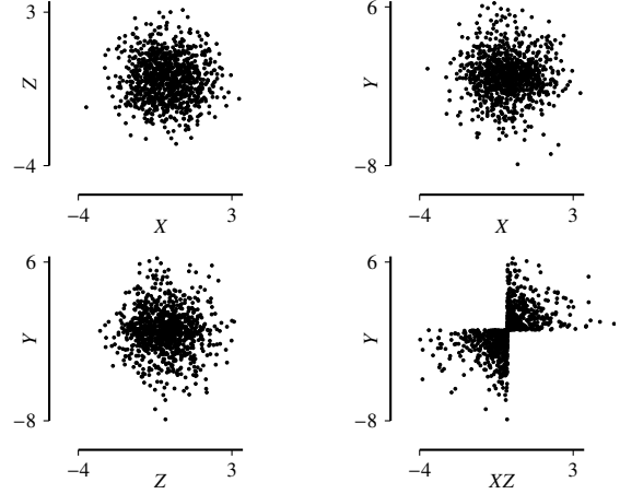
Figure 2: Sample data for the collider graph X \rightarrow Y \leftarrow Z , where X, Z \sim N(0, 1) are iid and Y := \text{sign}(XZ) \cdot E , with E \sim \text{Exp}(\frac{1}{\sqrt{2}}) . The dependence is only detectable by considering all three variables jointly.
