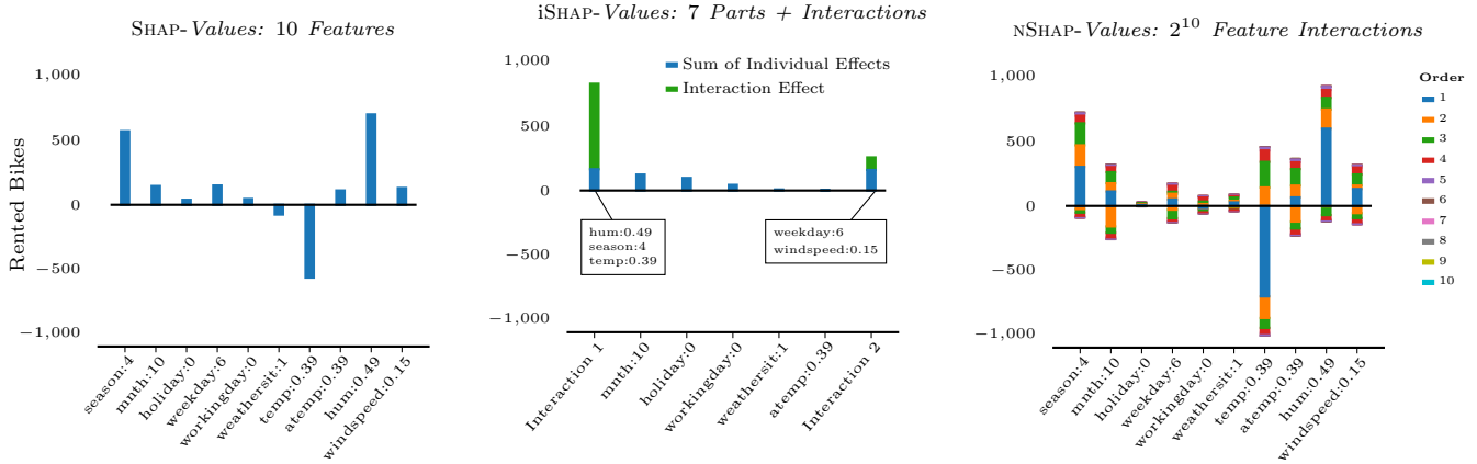
Figure 1: Comparison of SHAP (left), our approach iSHAP (middle) and NSHAP (right) on the Bike Sharing dataset (Fanaee-T & Gama, 2013). SHAP does not inform about any interactions, while NSHAP overflows with information. iSHAP provides a concise explanation for the high predicted demand: its is a warm and dry day for winter ( Season:4 , Hum:0.49 and Temp:0.39 ) and a Saturday with little wind ( Weekday:6 and Windspeed:0.15 ).
