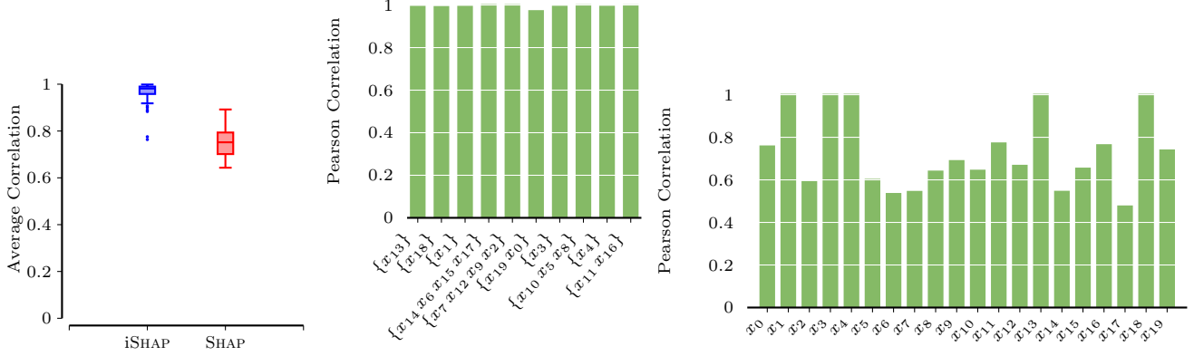
Figure 5: Comparison between ground truth feature importance (gradient times feature values) and the respective iSHAP values and SHAP values. On the left, we show the average correlation over all models. In the middle, we show the correlation between the iSHAP values and the ground truth for a specific model, on the right, we show the correlation between the ground truth and the SHAP values.
