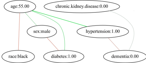
Figure 2: Interaction graph for predicted survival of a hospitalized COVID-19 patient. The detrimental effect of diabetes and hypertension on survival is alleviated by the relatively young age (55) of the patient.
