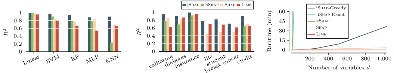
Figure 4: R^2 for surrogate models of iSHAP, nSHAP, SHAP and LIME across different model classes (left) and datasets (middle). iSHAP provides the most accurate surrogate model across all model classes and datasets, whilst scaling to more dimension than nSHAP (right).
