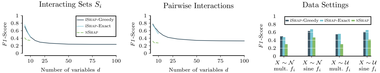
Figure 3: [Higher is better] F1 scores of recovered interactions in GAMs. iSHAP is more accurate than nSHAP in detecting full sets of interacting features (left) and pairwise interactions (middle), and can do so on more features. iSHAP-Greedy is equivalent to iSHAP-Exact and outperforms nSHAP across all data settings(right).
